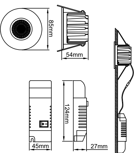
Fig. 1 80mm minimum void depth
