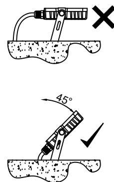
Ground Installation
